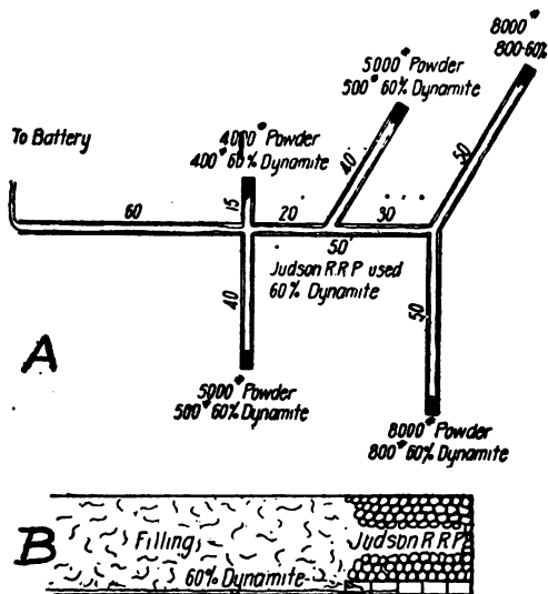
Fig. 104-A. Plan of Tunnels for Blasting.
